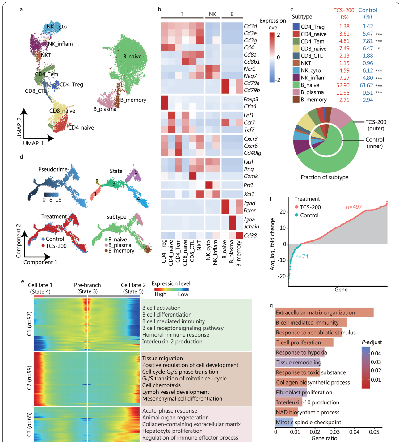
Fig. 6 Dynamic regulation of lymphocytes after TCS treatment.
