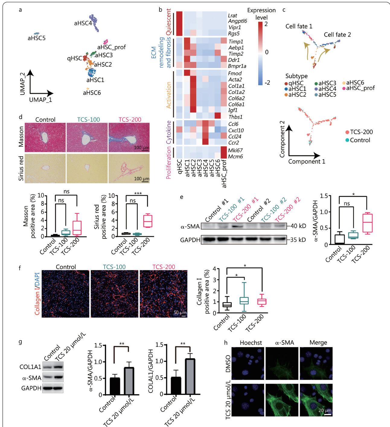
Fig. 4 Transcriptomic roadmap of HSCs activation.
