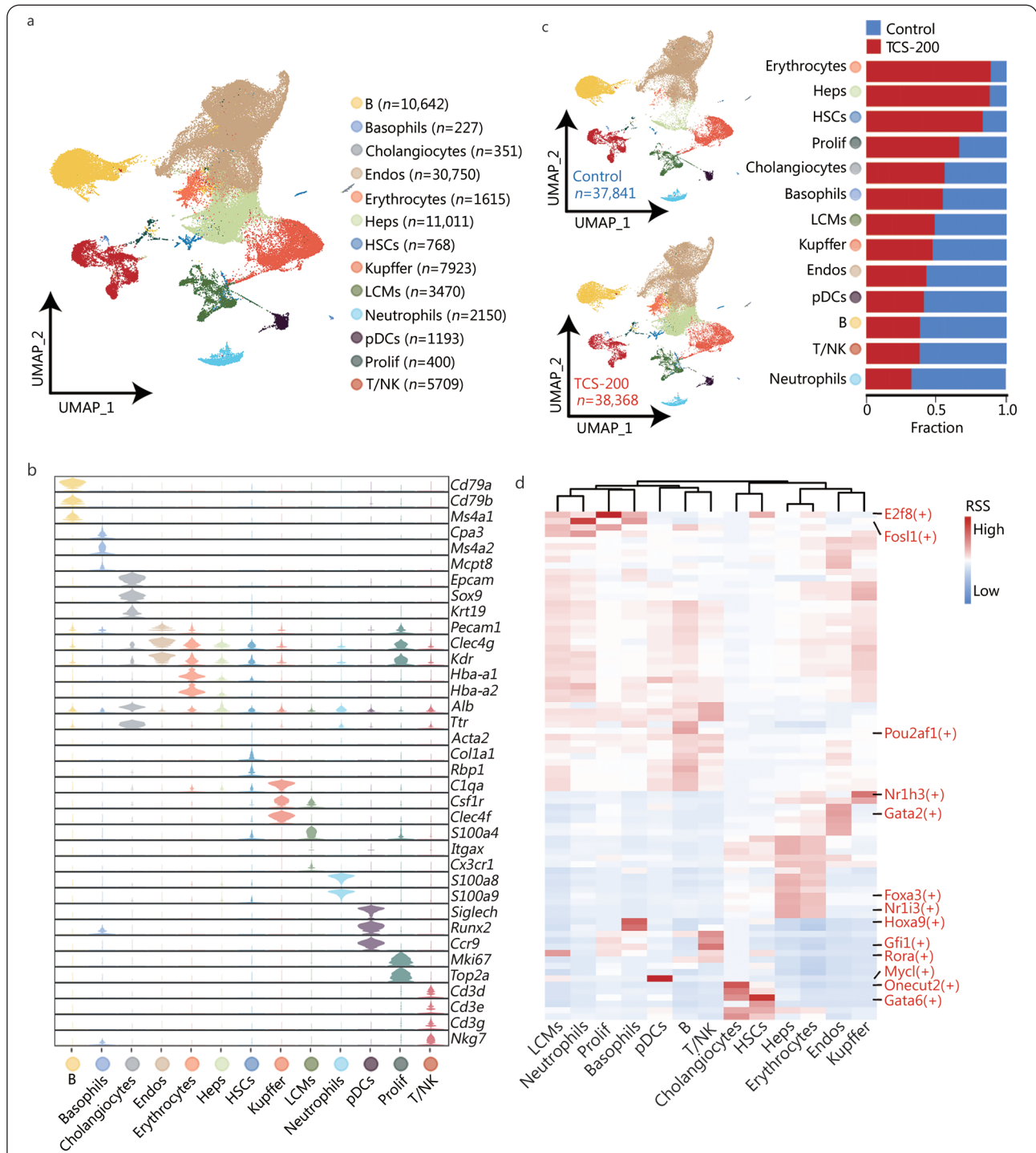
Fig. 2 Cell diversity in mice liver cells delineated by single-cell transcriptome.
